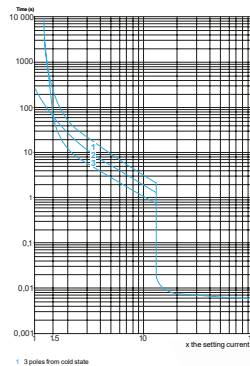
Kioldási jelleggörbe / Tripping characteristic
